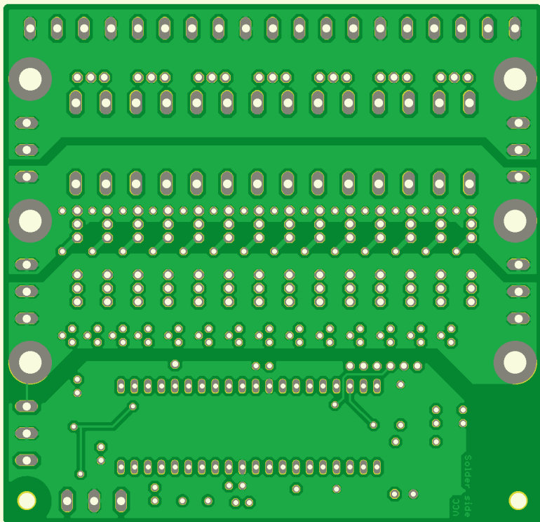
E652026 PCB view BOTTOM (bottomview)
