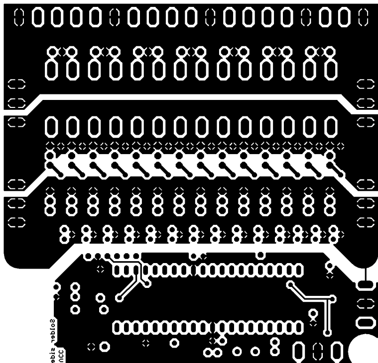
E652026 BOTTOM layer Image (topview)
