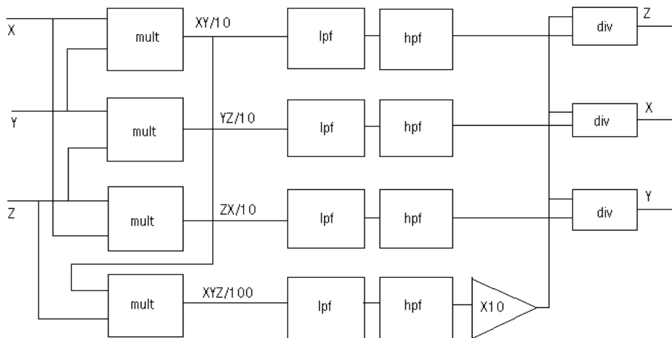
Carrier independent doppler demodulation circuit for invisible instrument Prof.Dr.Godfried-Willem RAES
